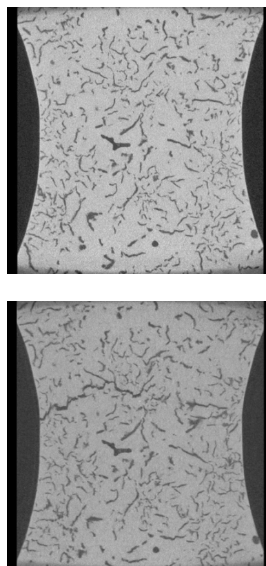
Figure. 2D slices extracted from the 3D tomography images of the same sample with (lower) and without (upper) an initiated fatigue crack.
