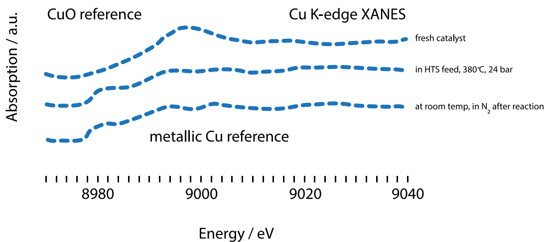
Figure 2 XAFS results from measurements on Cu promoted Cr stabilized Fe 3 O 4 under various industrial conditions. Ref: Puig-Molina et al., J. Phys. Chem. C, Vol. 114, No. 36, 2010.
